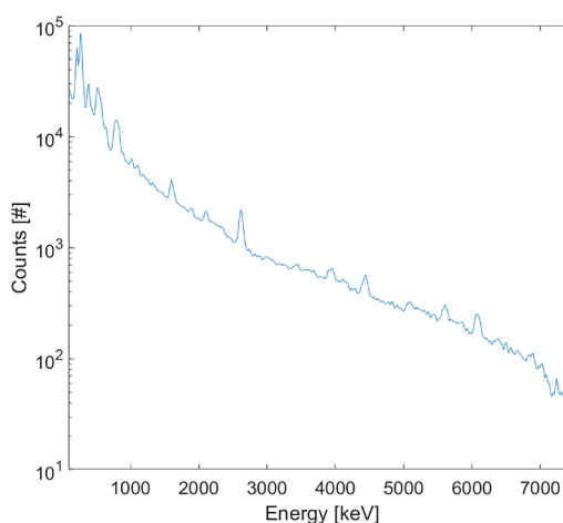
Gamma-ray spectrum from in-elastic neutron scattering from a narcotic simulant.
