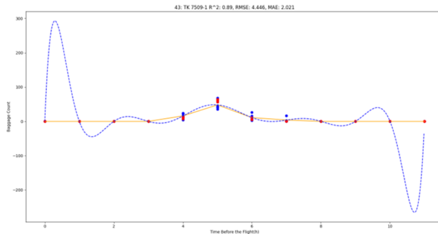
Figure. Hourly Baggage Prediction using Polynomial Regression Model
